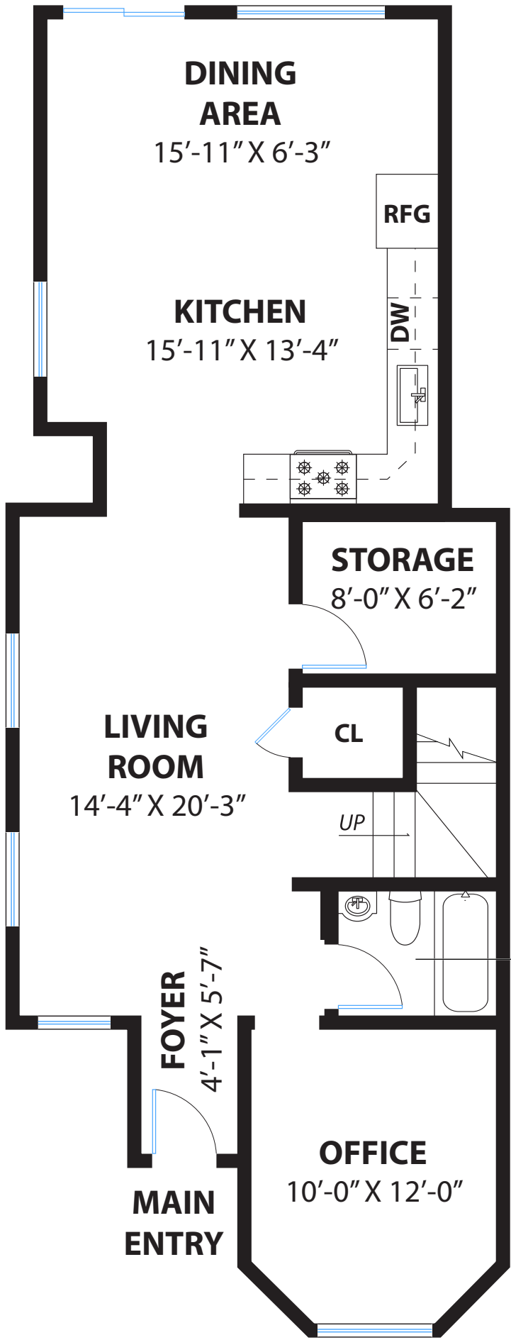
MAIN LEVEL
